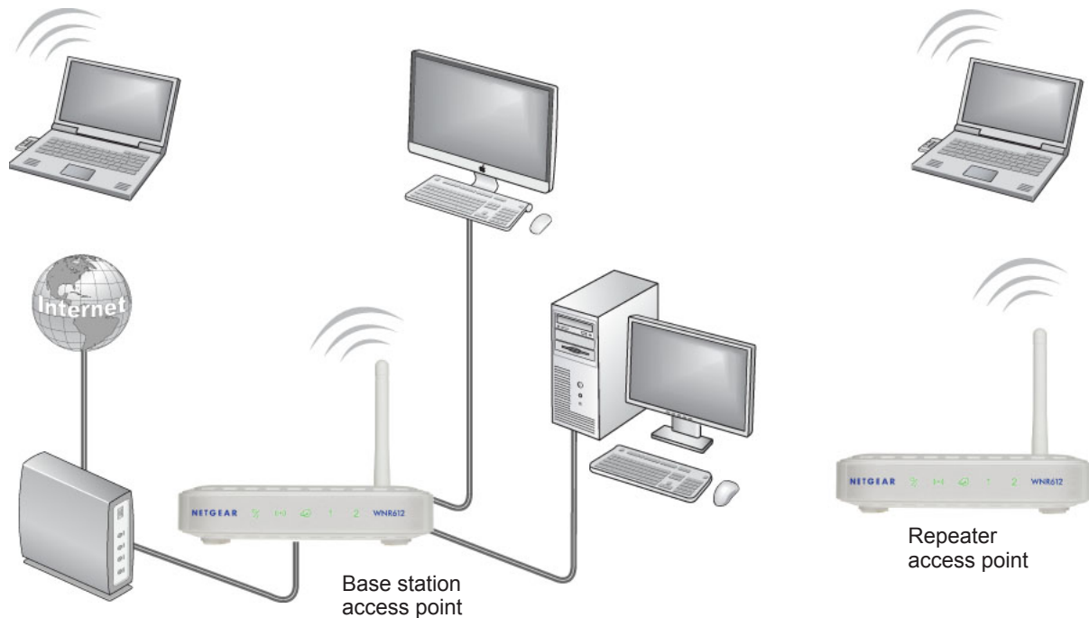
Figure 6. Wireless repeating scenario
